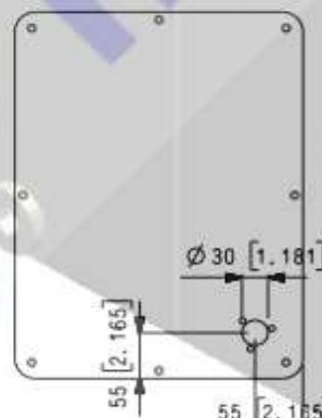
Style B Lid plate with Filler Breather (FB) cutout Lid
