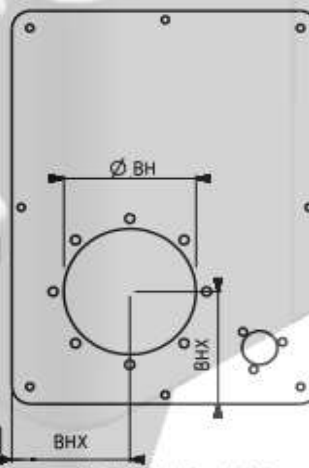
Style C Lid plate with Filler Breather (FB) and Return Filter (RF) cutout Lid
