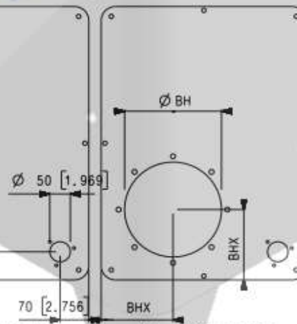
Style B Lid plate with Filler Breather (FB) cutout Lid
