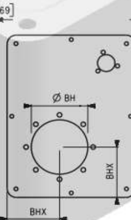
Style C Lid plate with Filler Breather (FB) and Bellhousing (BH) cutout Lid
